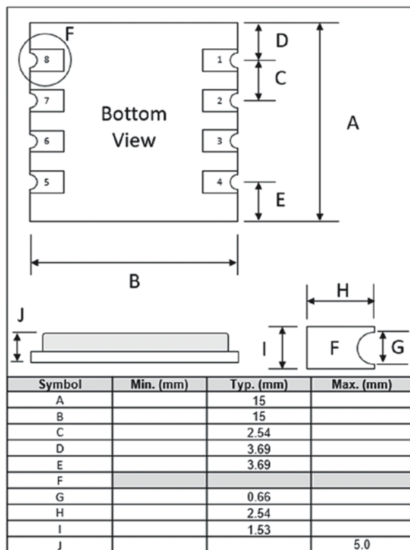
Component Footprint
